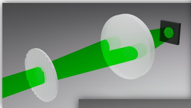
Interference ablation
